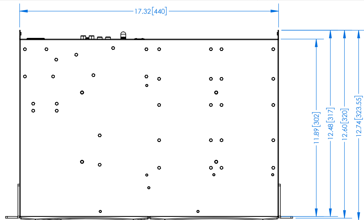
TOP VIEW
