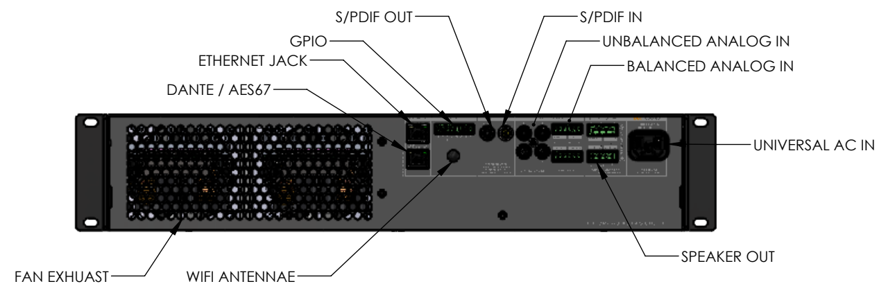
REAR VIEW
